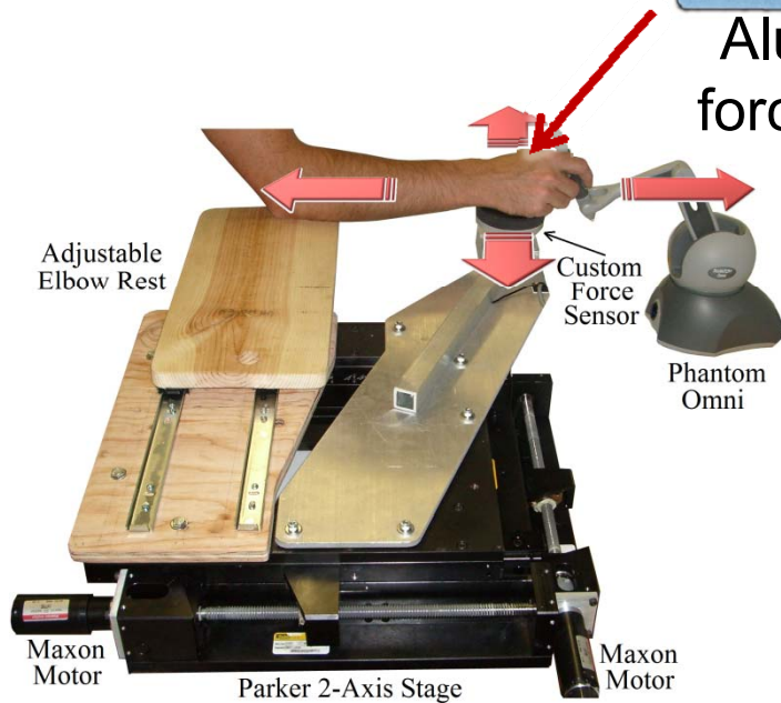
Active Handrest's extension plate and force sensor
