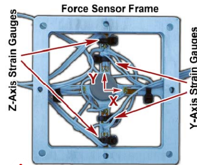
Aluminum force sensor
